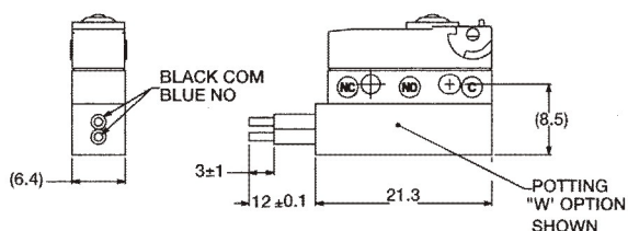
Z or W "B" WIRE ORIENTATION "C" CIRCUITRY
