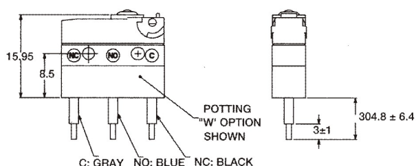
Z or W "A" WIRE ORIENTATION
