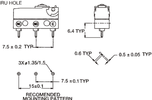
P PC THRU HOLE
