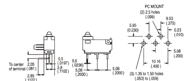
L LEFT FOOTED, PC THRU-HOLE
