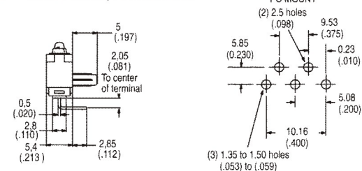
R RIGHT FOOTED, PC THRU-HOLE
